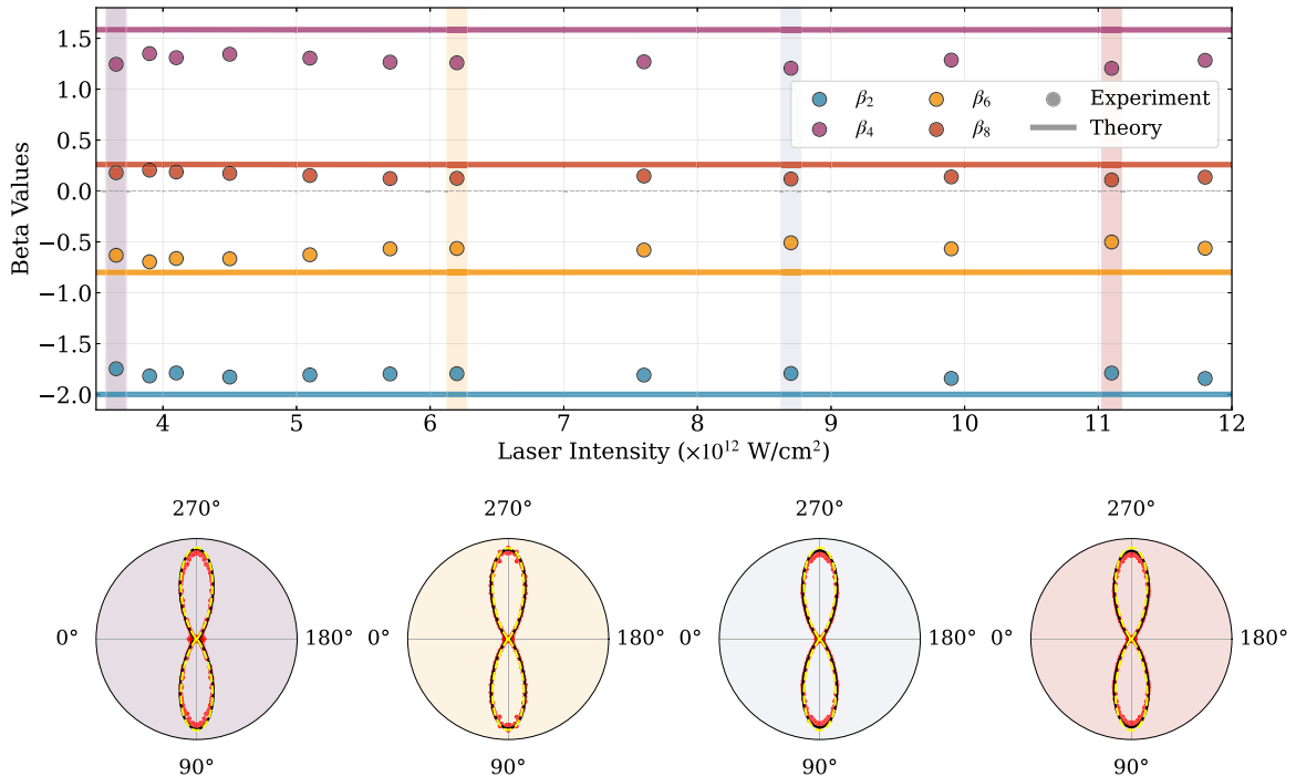
FIG. 2. Top: Beta parameters ( \beta_2 , \beta_4 , \beta_6 , \beta_8 ) as a function of laser intensity from 3.5 to 12 \times 10^{12} W/cm 2 for the ATI-1 peak in the corotating case. Experimental data (solid circles) obtained by averaging over all quadrant combinations are compared with theoretical predictions (lines). Colored vertical boxes indicate the intensities selected for a detailed polar-plot analysis. Bottom: Polar plots showing PADs at four representative intensities. The red points represent the experimental data, the black solid lines show experimental fits, and the yellow dashed lines are the relative theoretical predictions. The background colors correspond to the intensity markers in the top panel.
