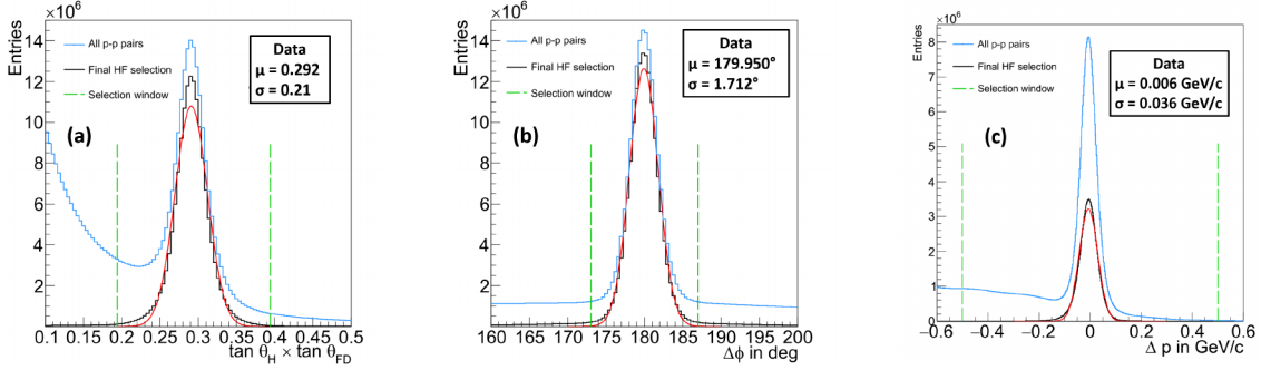
Figure 2: Distributions of (a) \tan\theta_H \times \tan\theta_{FD} , (b) \Delta\phi , and (c) \Delta p before (blue) and after (black) the selection cuts were applied to the other two variables. The green dashed lines show the selection window.
