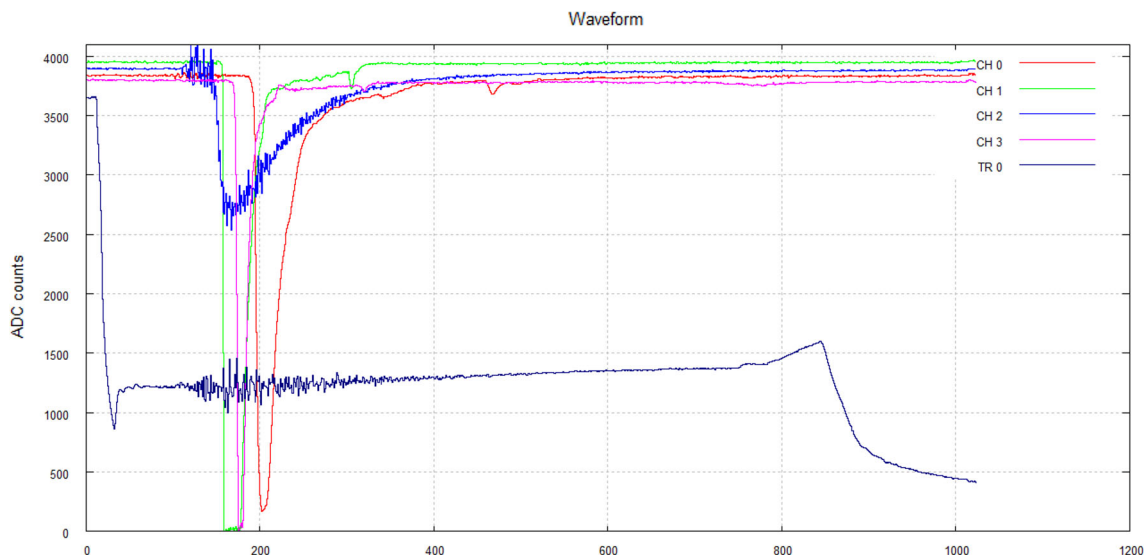
Fig. 13 Neutron TOF detection with different scintillators (see text for details)
