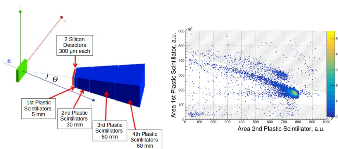
Fig. 14 Drawing of the detector (left) and \Delta E -E matrix (right); the dashed lines represent the conditions to select the scattered protons
