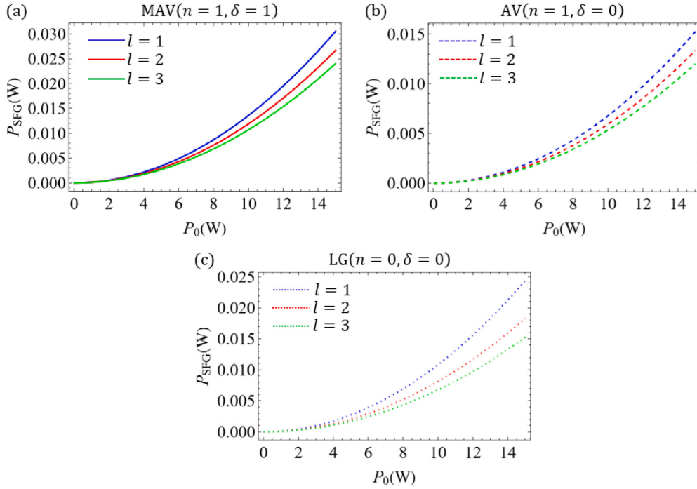
Fig. 7. Comparison of the SFG beam power as a function of the fundamental beam's power for TCs l = 1, 2 , and 3 . The results are presented in (a) for an MAV beam with parameters n = 1 , \delta = 1 ; in (b) for a traditional AV beam with parameters n = 1 , \delta = 0 ; and in (c) for an LG beam with parameters n = 0 , \delta = 0 . A similar trend in the SFG beam power is observed across all three beam types.
