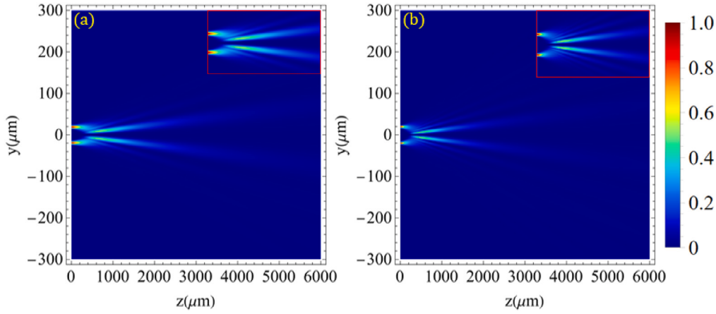
Fig. 12. Longitudinal intensity distributions of the SFG wave. In (a) l_1 = l_2 = 1 , n_1 = n_2 = 4 , \delta_1 = \delta_2 = 1 , and in (b) l_1 = l_2 = 1 , n_1 = n_2 = 10 , \delta_1 = \delta_2 = 1 . For higher beam order values, the self-focusing region shifts closer to the beam waist plane. The intensity colorbar is normalized to the respective maximum value for each panel.
