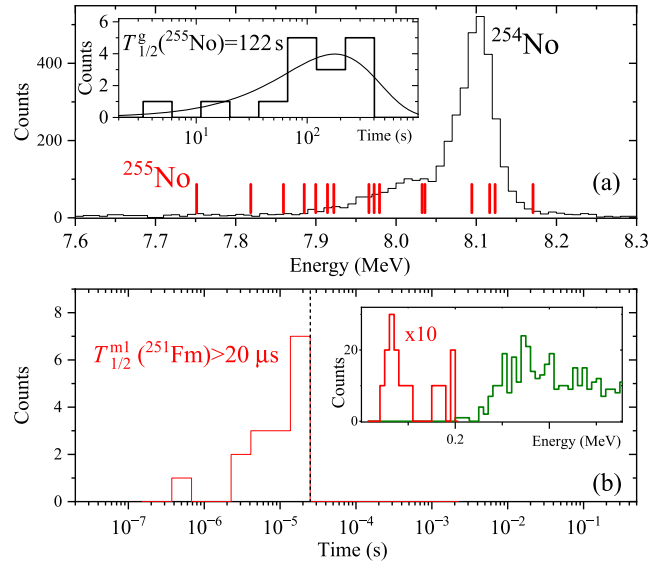
Fig. 5. (a) The energies of \alpha events observed in coincidence with delayed CEs, and thus assigned to originate from ^{255}\text{No} , are shown alongside the total beam-off \alpha spectrum from the ^{48}\text{Ca} + ^{208}\text{Pb} reaction. The time distribution of these \alpha events correlated with ERs, along with the corresponding fit, is presented in the inset of panel (a). Panel (b) also shows the time distribution of CEs relative to the preceding \alpha signals. A comparison of the CE energy distribution with that of random events is shown in the inset of panel (b). For details, see text.
