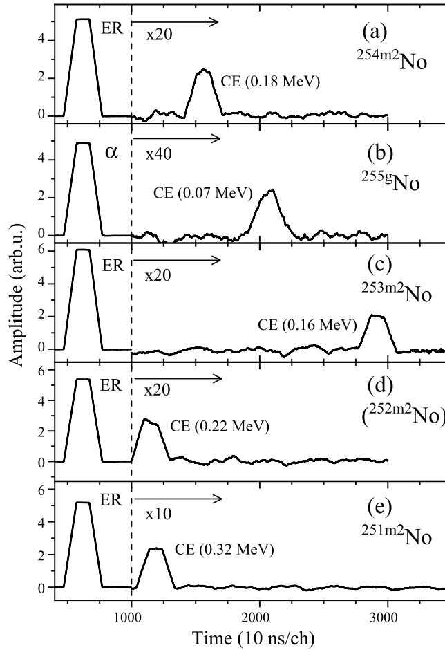
Fig. 4. Examples of trapezoidal filtered ER and \alpha traces from X strips, where delayed CEs originating from \mu s-isomers from No and Fm isotopes are shown. To highlight the low-energy CE signals, the amplitudes after ERs are shown with different amplification factors.
