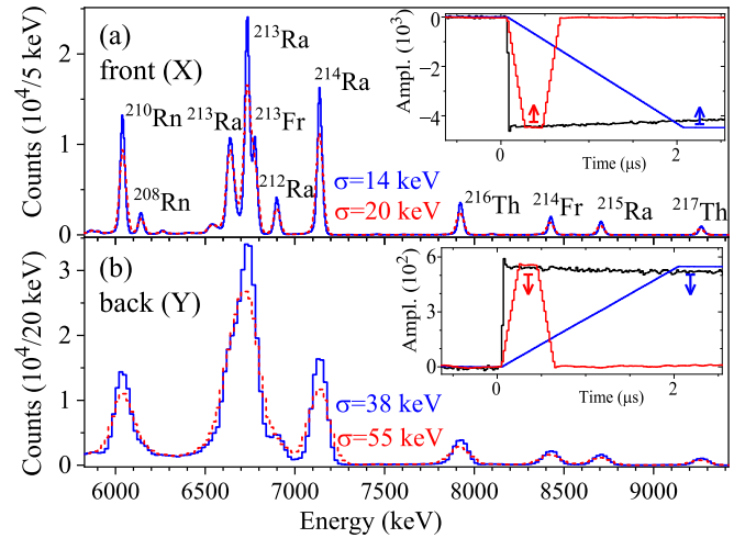
FIG. 1. Summed energy spectra of beam-off events measured in 192 X (a) and 72 Y (b) strips from the ^{48}\text{Ca} + ^{174}\text{Yb} reaction. The calibrated energies based on signal-amplitudes extracted from two different trapezoidal filters are shown. Insets show the shapes of 7 \text{ MeV} signals and their shapes after two different trapezoid filters (one with a base of 700 and flat top of 500 samples and the other with 30 and 10 samples for base and flat top, respectively [34]. Arrows mark the positions where average amplitudes of four samples were used for the energy calibrations. The energy resolutions ( \sigma ) are given for the peak corresponding to the \alpha decay of ^{214}\text{Ra} . See text for details.
