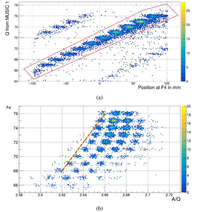
Fig. 2. (a) Q from first MUSIC plotted as function of the x position at F4. Three diagonal bands represent, from top to bottom, (1-0), (0-0) and (0-1) charge states respectively. Selection of (0-0) is shown. (b) Particle identification plot for the ^{190}\text{Lu} setting using time of flight calibration parameters. The orange line indicates the expected position of the Z-1, A-3 isotope sequence starting from ^{202}\text{Os} .
