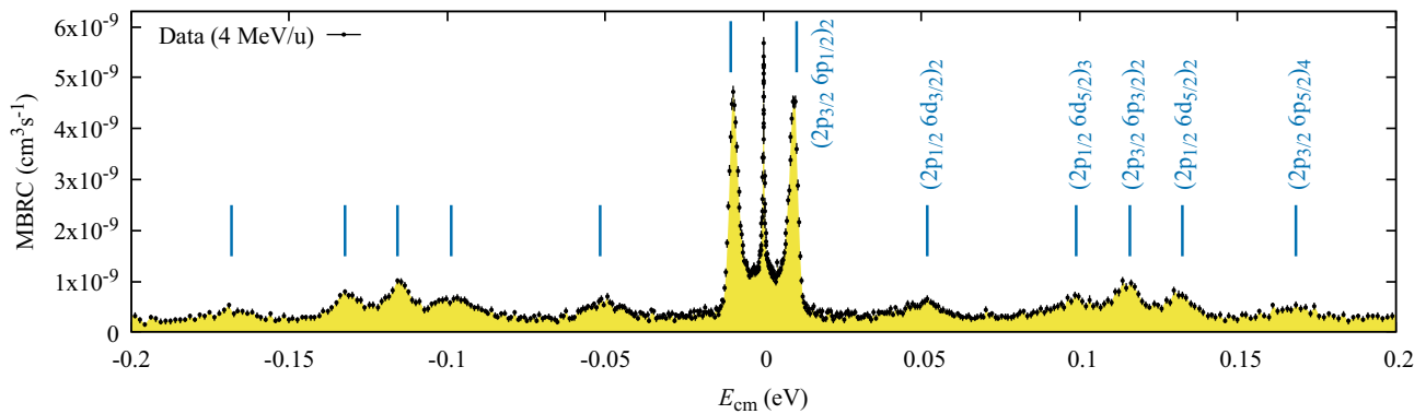
Fig. 3 Example of a measured recombination rate coefficient for F^{6+} + e \rightarrow F^{5+} at lowest energies. Negative or positive values of E_{cm} represent electron–ion collisions with \beta_e < \beta_i or \beta_e > \beta_i , respectively. The labels indicate expected DR resonance energies as per Tokman et al., 2002 [34], and Lestinsky, 2007 [35]
