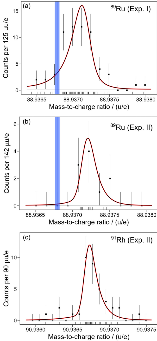
FIG. 3. Measured mass spectra of ^{89}\text{Ru} in Experiment I (a), in Experiment II (b) and of ^{91}\text{Rh} in Experiment II (c). The square symbols are the binned data used just for representation; the fit was obtained using unbinned data, which are shown as a rug graph at the bottom of each panel. The solid red curve shows the fitted Hyper-EMG probability distribution function, normalized to the number of events in the histogram. In panels (a) and (b), the blue line represents the literature mass value of ^{89}\text{Ru} and the blue shadow represents the literature mass uncertainty [45], where the width corresponds to \pm one standard deviation.
