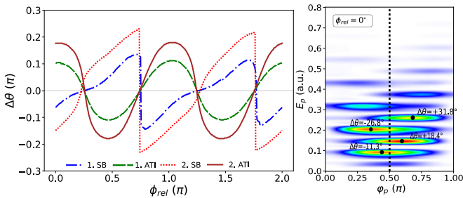
FIG. 5. Phase-dependent angular deflection of photoelectron peaks. Left: Angular shifts \Delta\theta of the first and second ATI peaks and corresponding SB as a function of the relative phase \phi_{rel} . Right: Photoelectron momentum distribution at \phi_{rel} = 0^\circ , illustrating the definition of the angular shift \Delta\theta relative to the reference direction \varphi_{ref} = \pi/2 (vertical dashed line). The marked points correspond to the peak positions used to extract \Delta\theta for different ATI and SB orders. The other parameters are the same as in Fig. 2.
