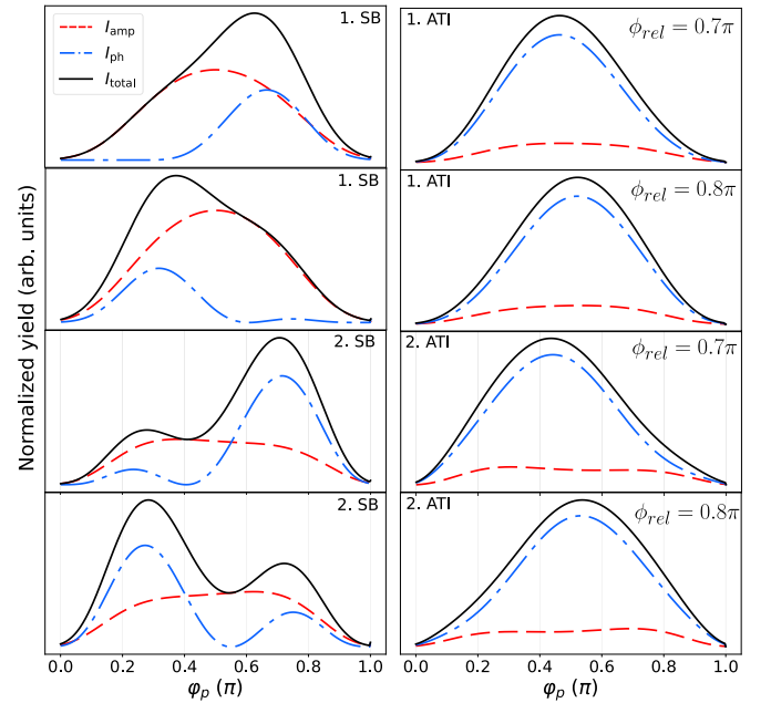
FIG. 7. The calculated yield of amplitude modulation I_{amp} (red dashed lines) and phase modulation I_{ph} (blue dash-dotted lines) for the first two sidebands and above-threshold-ionization peaks. The black solid lines represent the total yield for each peak. All other parameters are the same as Fig. 6 but for \phi_{rel} = 0.7\pi and 0.8\pi . The vertical axis shows the normalized yield and ranges from 0 to 1. Within each panel, the amplitude, phase, and total yields are normalized using the same maximum value of the total yield.
