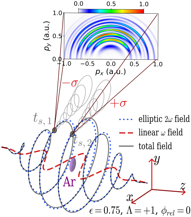
FIG. 1. Illustration of the two-color strong-field ionization mechanism considered in this work. The driving field consists of a strong elliptically polarized 2\omega field of intensity 1.42 \times 10^{14} W/cm 2 , shown by the blue dotted curve, and a weak linearly polarized \omega field of intensity 8.8 \times 10^{11} W/cm 2 , shown by the red dashed curve. Their coherent superposition gives the total electric field, indicated by the gray solid curve, which ionizes the Ar atom near adjacent subcycle field maxima. The two emitted electron wave packets, launched at the saddle times t_{s,1} and t_{s,2} , acquire opposite weak-field-induced modulation phases, denoted by -\sigma and +\sigma . The inset shows the resulting photoelectron momentum distribution in the polarization plane, where the subcycle phase modulation leads to angular deflections of the emitted electron signal. The field parameters are \epsilon = 0.75 , \Lambda = +1 , and \phi_{\text{rel}} = 0 .
