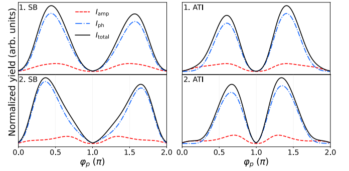
FIG. 6. The calculated yield of amplitude modulation I_{amp} (red dashed lines) and phase modulation I_{ph} (blue dash-dotted lines) for the first two sidebands (left column) and ATI peaks (right column) in the two-color field composed of an elliptically polarized 400-nm pulse and a weak linearly polarized 800-nm field. The black solid lines represent the total yield for each peak. We also consider \phi_{rel} = 0^\circ . The vertical axis shows the normalized yield and ranges from 0 to 1. Within each panel, the amplitude, phase, and total yields are normalized using the same maximum value of the total yield.
