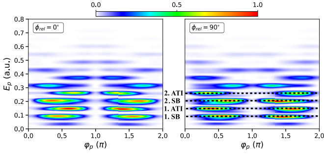
FIG. 4. Photoelectron momentum distributions in the polarization plane as a function of emission angle \varphi_p and energy E_p for relative phases \phi_{rel} = 0^\circ (left) and 90^\circ (right) calculated using SFA. The other parameters are the same as Fig. 2. The spectra display ATI peaks and SBs, indicated by dashed lines. The color scale denotes the normalized yield.
