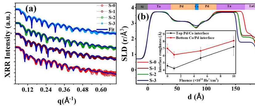
Fig. 1. (a) X-ray reflectivity (XRR) signals for all the samples presented in this study, the symbols are the experimental data, and the continuous blue line shows the best fit to each datum. (b) Scattering length density (SLD) profile showing depth-dependent electron density variations for each sample; the inset shows the variation of top Pd/Co and bottom Co/Pd interfacial roughness as a function of fluence.
