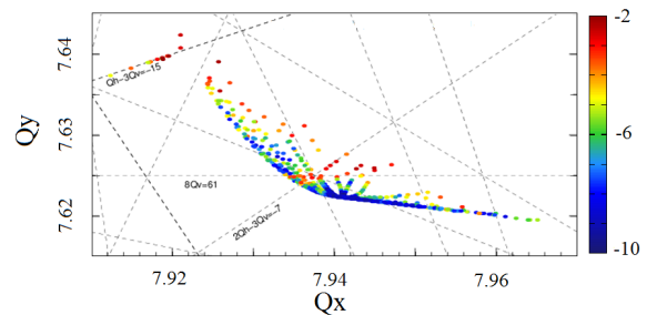
Figure 2: Frequency diagram for modified optics
