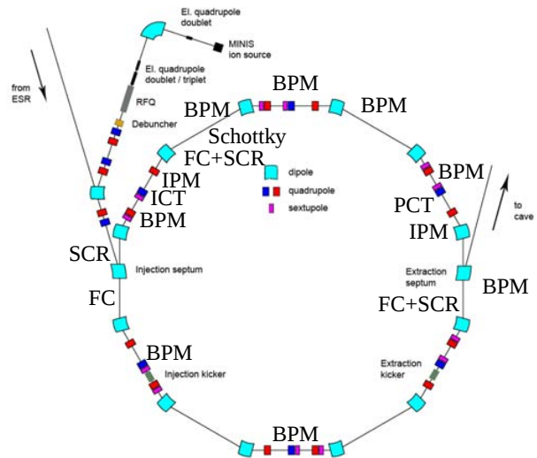
Figure 1: Layout and Diagnostics of CRYRING@ESR.
