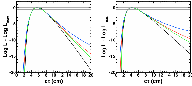
Fig. 1. (Color online.) The likelihood function of the data set shown in [9] with the different extrapolations based on Gaussian function of {}^3_{\Lambda}\text{H} and of {}^4_{\Lambda}\text{H} in left and right panel respectively. The red curves correspond to the real likelihood function obtained from the dataset. The blue and black curves correspond to the Gaussian function with linear standard deviation and with linear variance respectively. The green curve is the average combination of the two curves.
