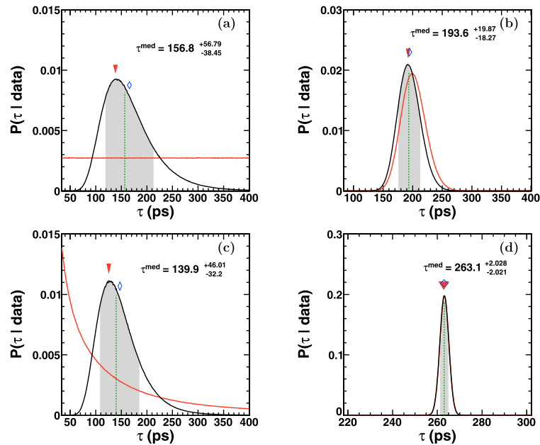
Fig. 4. (Color online.) Posterior distributions for the {}^4_{\Lambda}\text{H} data set with the same configuration of Fig. 3.
