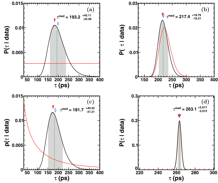
Fig. 3. (Color online.) Posterior distributions for the {}^3_{\Lambda}\text{H} data set, panel (a) for the uniform prior, panel (b) for the previous measurements prior, panel (c) for the Jeffreys prior and panel (d) for the \Delta prior. In each panel the posterior distribution is displayed in black line while the prior distribution is in red line.
